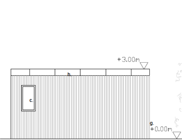
West Elevation As Proposed
