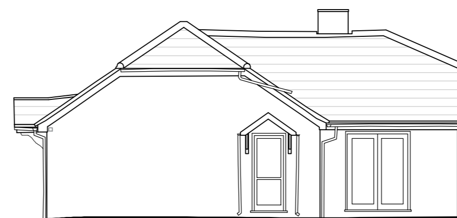
EXISTING SIDE ELEVATION 1
