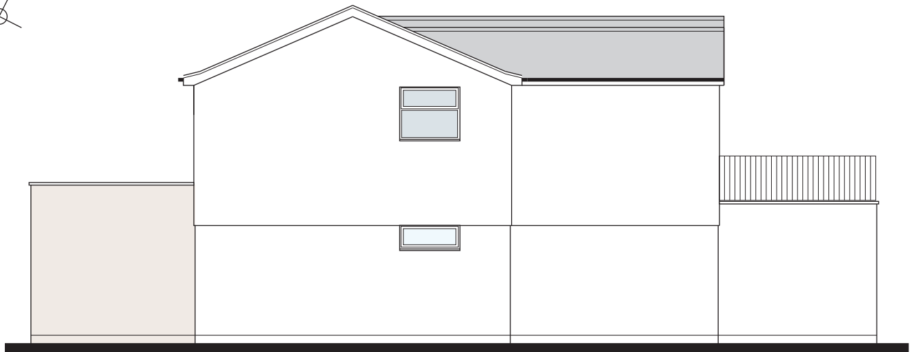
Side Elevation
