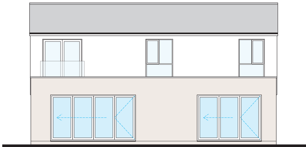
Rear Elevation
