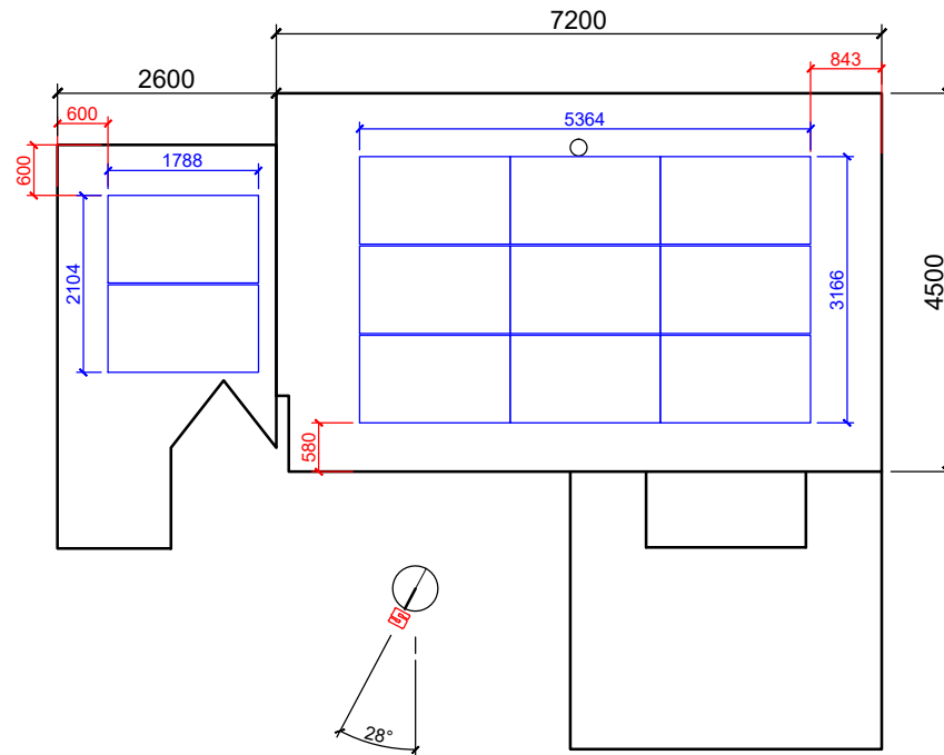
11 panel PV array: Option D: 4.18 kWp of LG Neon monocrystalline 380W panels
