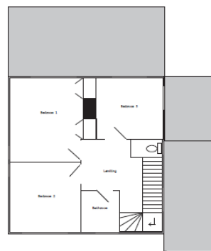
EXISTING FIRST FLOOR LAYOUT
