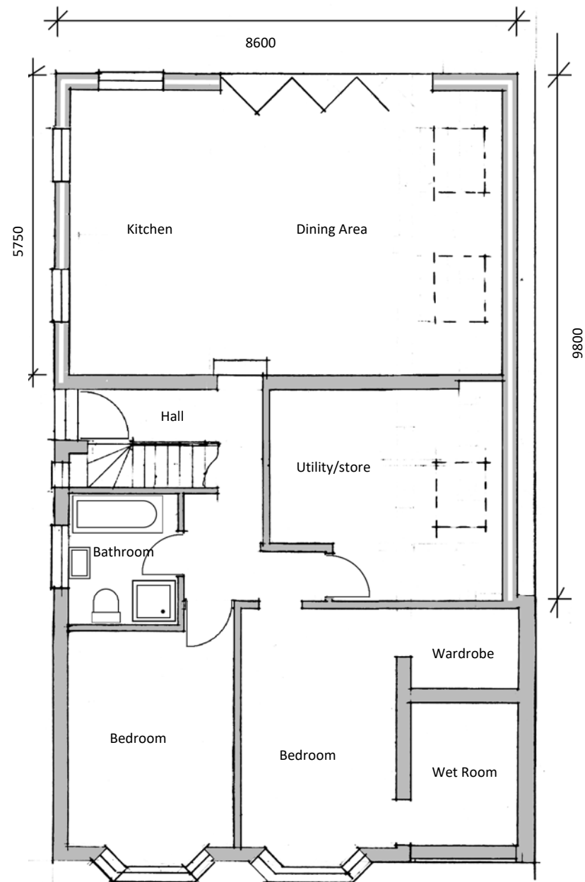
GROND FLOOR PLAN
