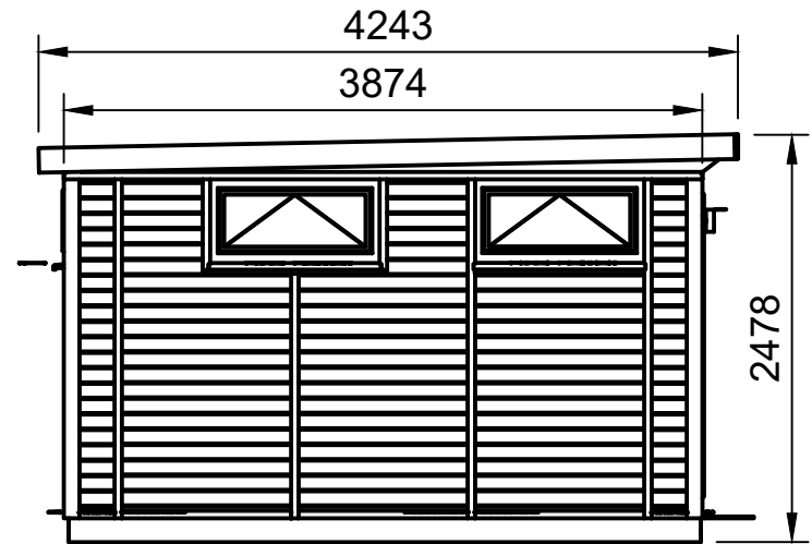
Left Elevation
