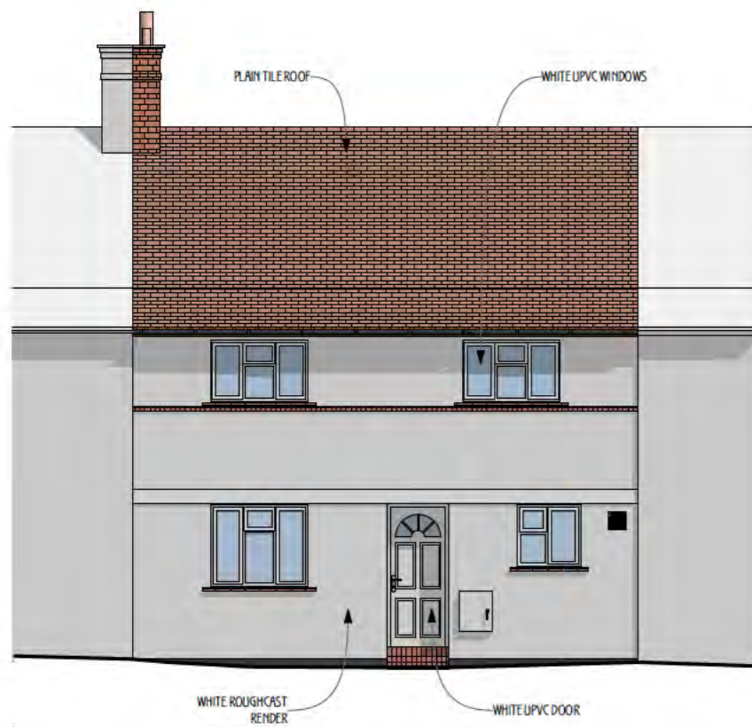
E-01 South East Elevation 1:100
