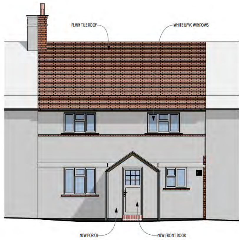
E-01 South East Elevation 1:100
