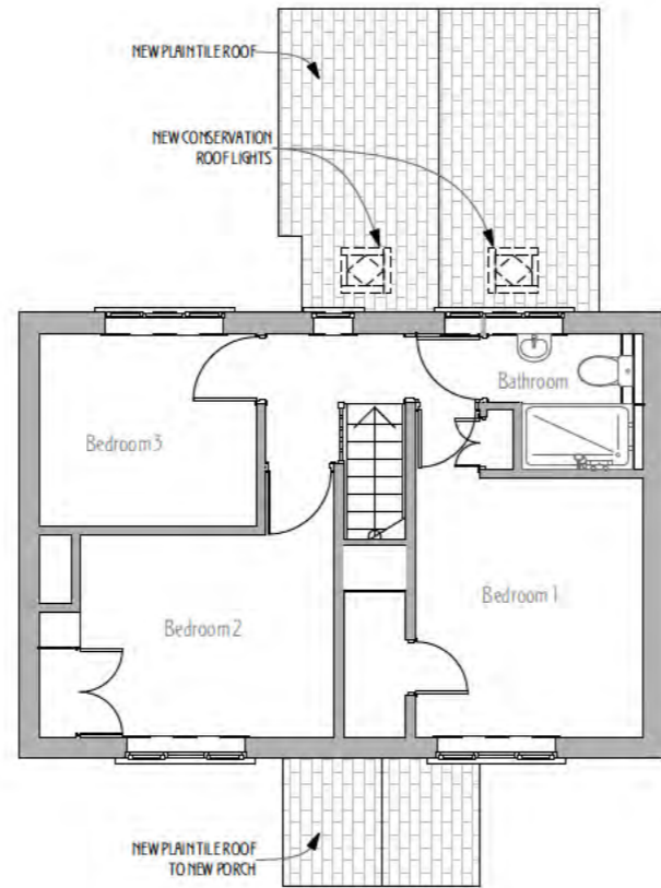
FF First Floor Plan 1:100
